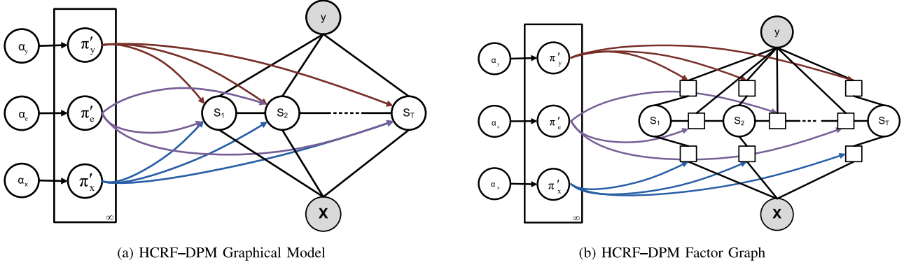
Fig. 1. Graphical representation of our Variational IHCRF driven by a number of Dirichlet processes incorporated in the model potentials.
