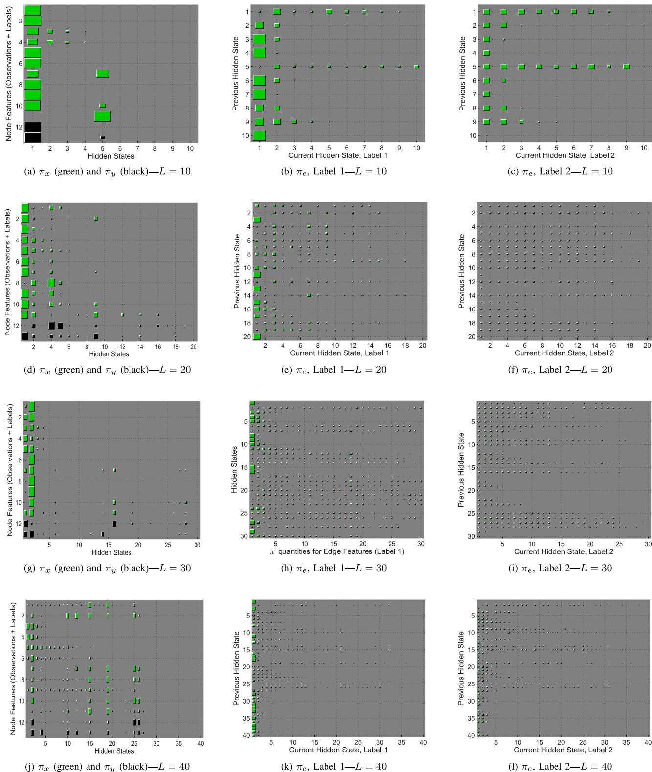
Fig. 3. Hinton Diagrams of \pi -quantities in node and edge features of variational HCRF-DPM models with L = 10 on the first row (a-c), L = 20 on the second (d-f), L = 30 on the third (g-i), L = 40 on the fourth (j-l) for ADA2. The first column presents the \pi -quantities for node features: \pi_x for observation features in green, \pi_y for labels in black. The second and third columns present the \pi_e -quantities for labels 1 and 2 respectively. See text for additional details.
