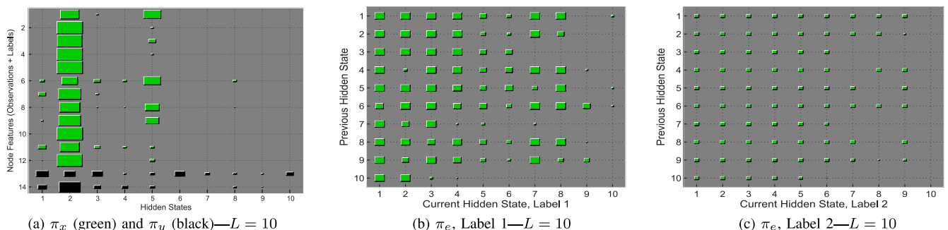
Fig. 5. Hinton Diagrams of \pi -quantities in node and edge features of variational HCRF-DPM models with L = 10 for PAIN2. The first column presents the \pi -quantities for node features: \pi_x for observation features in green, \pi_y for labels in black. The second and third columns present the \pi_e -quantities for labels 1 and 2 respectively. See text for additional details.
