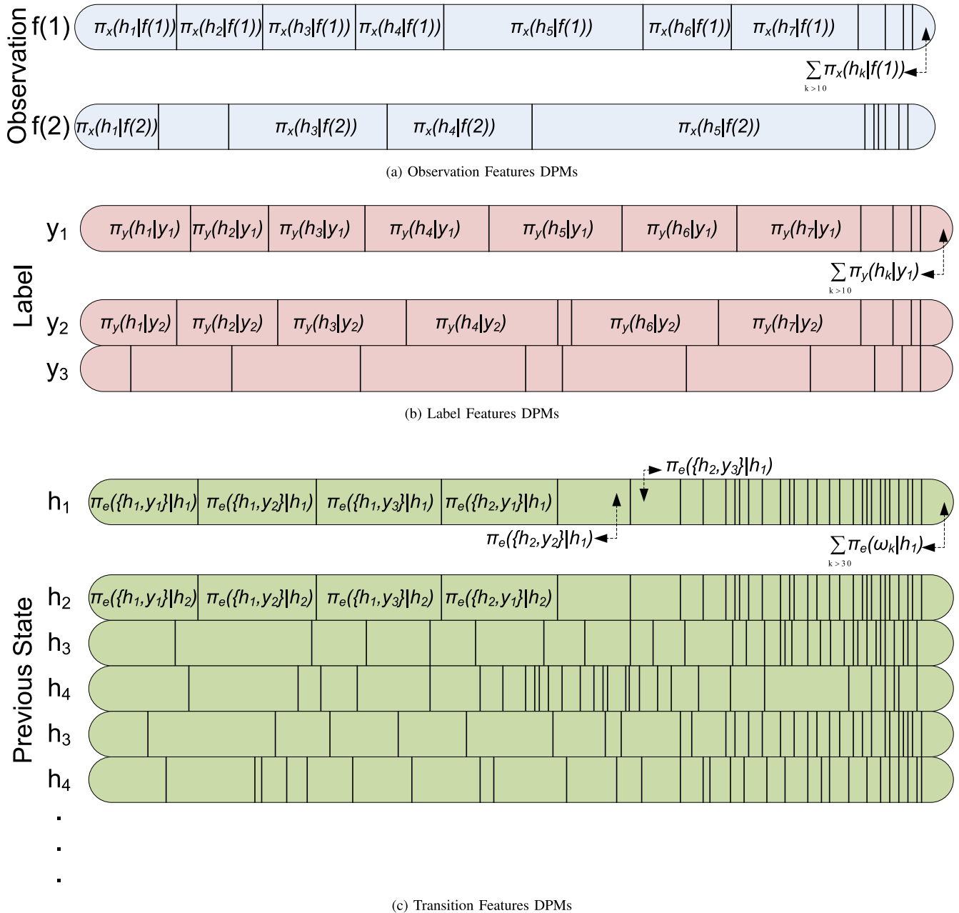
Fig. 2. Visualization of the \pi -‘sticks’ used to construct the infinite states in our HCRF-DPM. The fictitious model presented here has two observation features f(1), f(2) , 3 labels y_1, y_2, y_3 and fewer than 10 important hidden states h_1, h_2, h_3 \dots . Each ‘stick’ sums up to 1, and the last piece always represents the sum of the lengths that correspond to all hidden states after the 10th state. Notice that for the \pi_e -‘sticks’ this corresponds to 30 \omega states. For example \pi_e(h_1, y_3|h_2) controls the probability of transitioning from h_2 to h_1 in a sequence with label y_3 . See text for more details.
