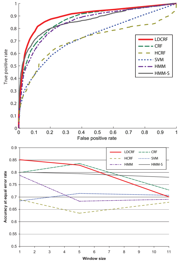
Figure 5. Results with AvatarEye dataset: (top) ROC curves for a window size of one; (bottom) Accuracy at equal error rates as a function of the window size.
