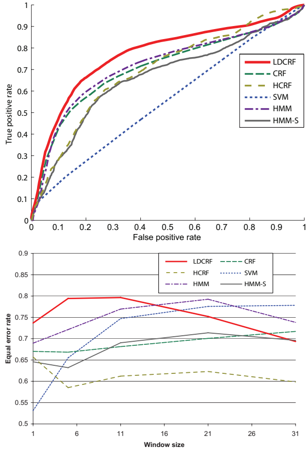
Figure 3. Results with WidgetsHead dataset: (top) ROC curves for a window size of one (no long range dependencies); (bottom) Accuracy at equal error rates as a function of the window size.
